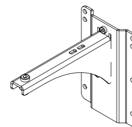
Wall mounting bracket VNI-WM200 VNI-WM280 VNI-WM330
