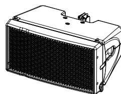
GEOM1025 Line array element, 2 way passive, 1 x 10 inches, touring, black, 25° vertical, 80° horizontal, 59 Hz - 20 KHz, 131 dB, 21 Kg (GEO M1025-PW for white version)
