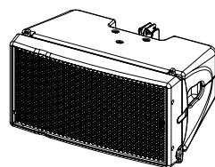
GEOM1012 Line array element, 2 way passive, 1 x 10 inches, touring, black, 12.5° vertical, 80° horizontal, 59 Hz - 20 KHz, 131 dB, 21 Kg (GEO M1012-PW for white version)
