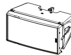
GEOM1025-I Line array element, 2 way passive, 1 x 10 inches, install, black, 25° vertical, 80° horizontal, 59 Hz - 20 KHz, 131 dB, 21 Kg (GEO M1025-IPW for white version)
