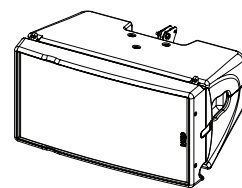
GEOM1012-I Line array element, 2 way passive, 1 x 10 inches, install, black, 12.5° vertical, 80° horizontal, 59 Hz - 20 KHz, 131 dB, 21 Kg (GEO M1012-IPW for white version)
