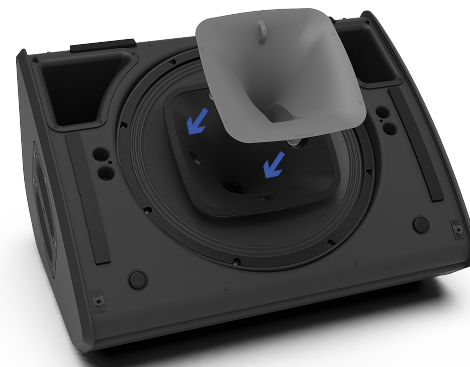
Grille removed, an additional magnetic flange can be quickly fitted to change directivity from 60°x60° to Asymmetrical
