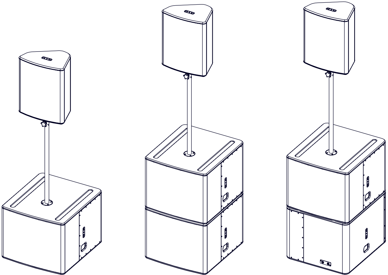
Stage monitor applications with Subs (OMNI or CARDIO modes)
