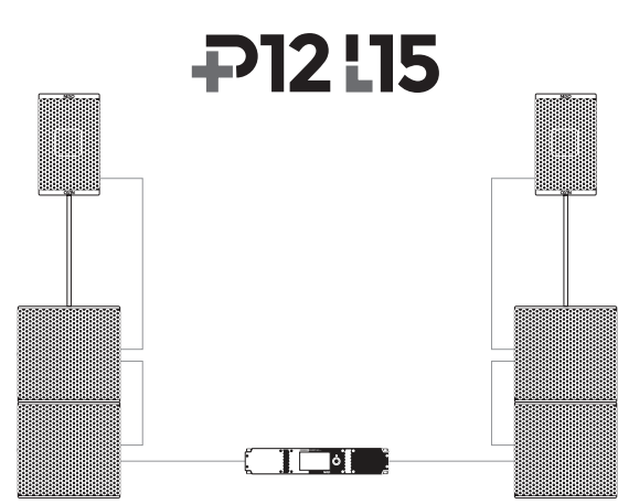
NXAMP4X2MK2 powering 1 X P12 and 2 X L15 per side
