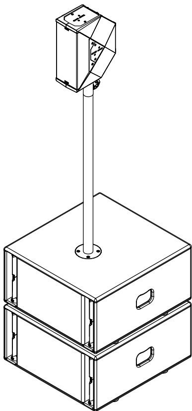
“OMNI” Assembly
