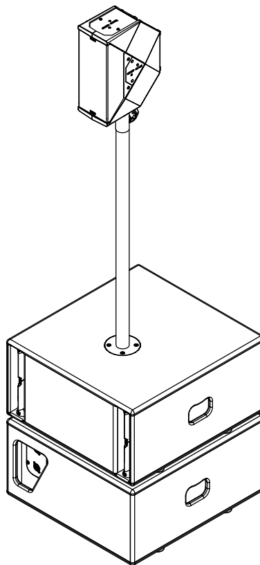
“CARDIO” Assembly
