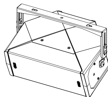
IDI-HBRK24 (only used on ID24 with the last 6 digits of the serial number \geq 200\ 000 ).
