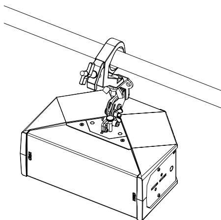
IDT-HBRK24 (only used on ID24 with the last 6 digits of the serial number \geq 200\ 000 ).
