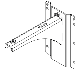
Wall mounting bracket
