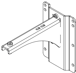
Wall mounting bracket
