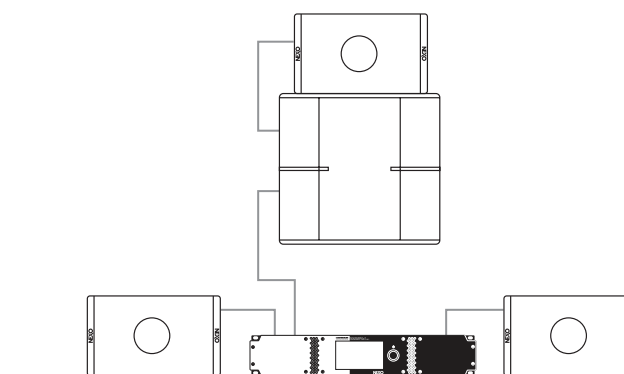
Monitor System: 1 x P10 Wedge on 1 x L15 Sub (Drum Fill) + 2 x P10 Wedges powered by NXAMP4X1MK2
