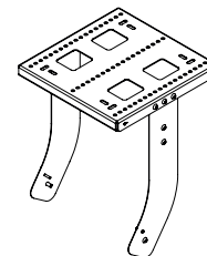
VNI-VCPL425 (ePS8 under eLS600) VNI-HCPL535 (ePS10 under eLS600) VNI-VCPL365 (ePS6 under eLS400) VNI-HCPL425 (ePS8 under eLS400) VNI-VCPL600 (ePS12 under eLS18) VNI-HCPL535 (ePS10 under eLS18) eLS and ePS clusters
